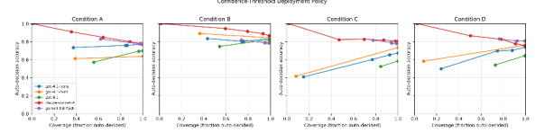
Figure 8: Confidence-threshold deployment policy, auto-decision accuracy vs. coverage for each model and condition.
