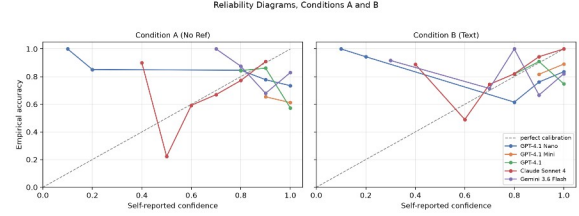
Finding 5: Claude is the best-calibrated verifier on all three measures, in every condition. This holds whether we bin coarsely (3 bins, matching elicitation) or finely (15 equal-mass bins), and is confirmed by the binning-free Brier score. Claude's near-perfect ECE_3bin (e.g., 0.015 in Condition A) loosens slightly under finer binning (ECE_15bin = 0.030) but remains lower than the next-best model in every condition.
