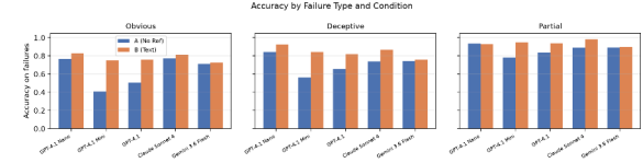
Figure 4: Accuracy by failure type (obvious, deceptive, partial) and condition, across all five models.
