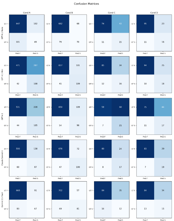
Figure 7: Complete confusion matrices for all five models across all four conditions.
