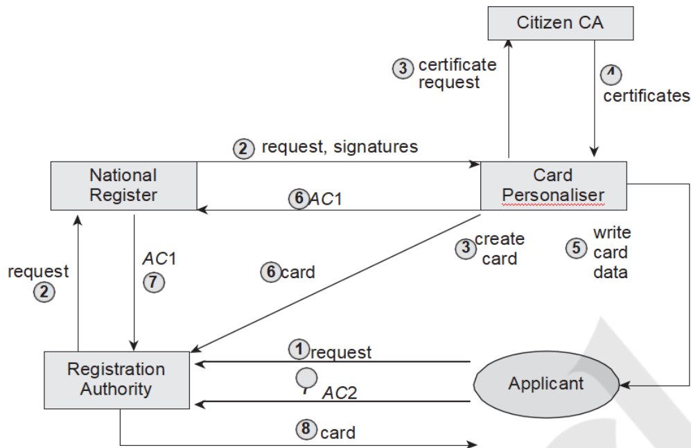
Figure 12.14. eID card issuing process
