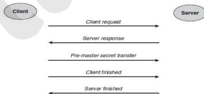
Figure 12.1. Simple SSL Handshake Protocol message flow
