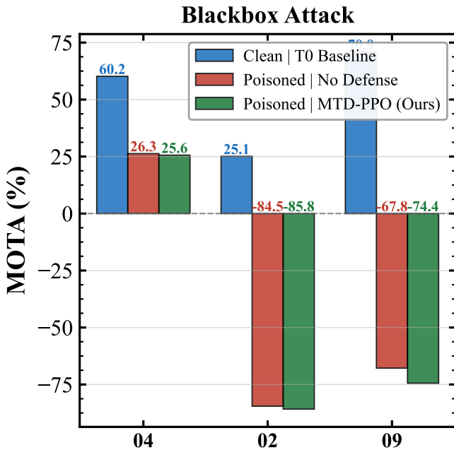
Fig. 2 — Per-Sequence MOTA Under Three Evaluation Conditions
