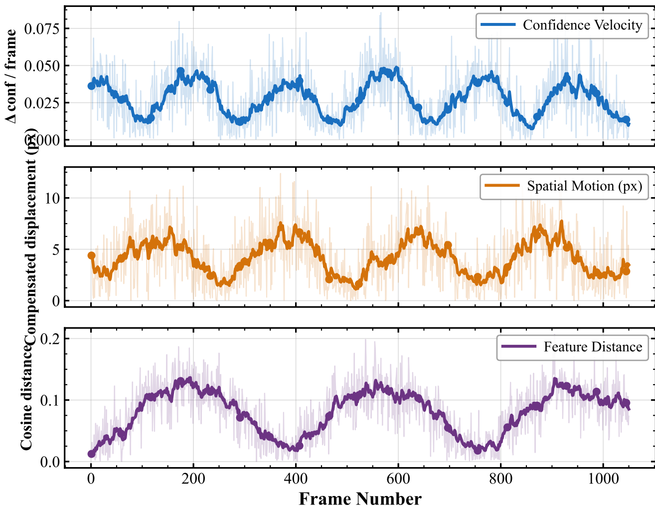
Fig. 7 — RL State Vector Dynamics (MOT17-04)
