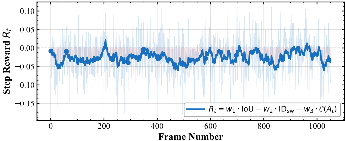
Fig. 9 — Step-wise Reward Signal During Inference
