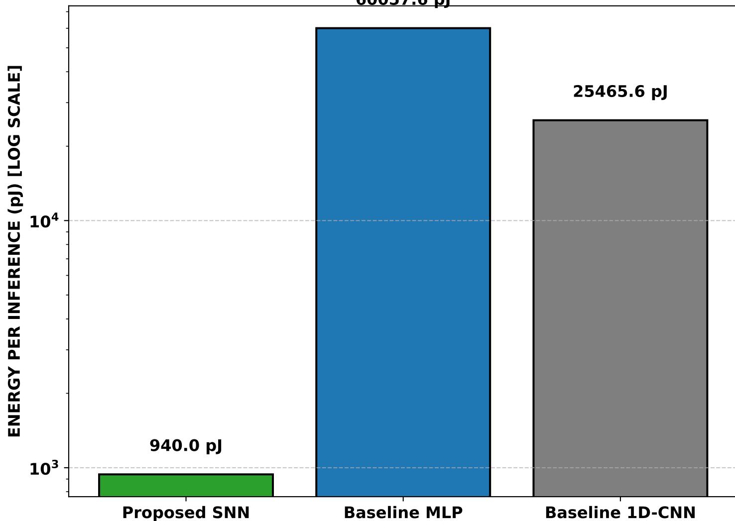
HARDWARE INFERENCE COST: SNN VS CONTINUOUS MODELS
