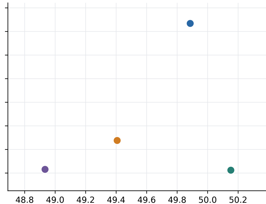
HSC-Behaviour-SD
