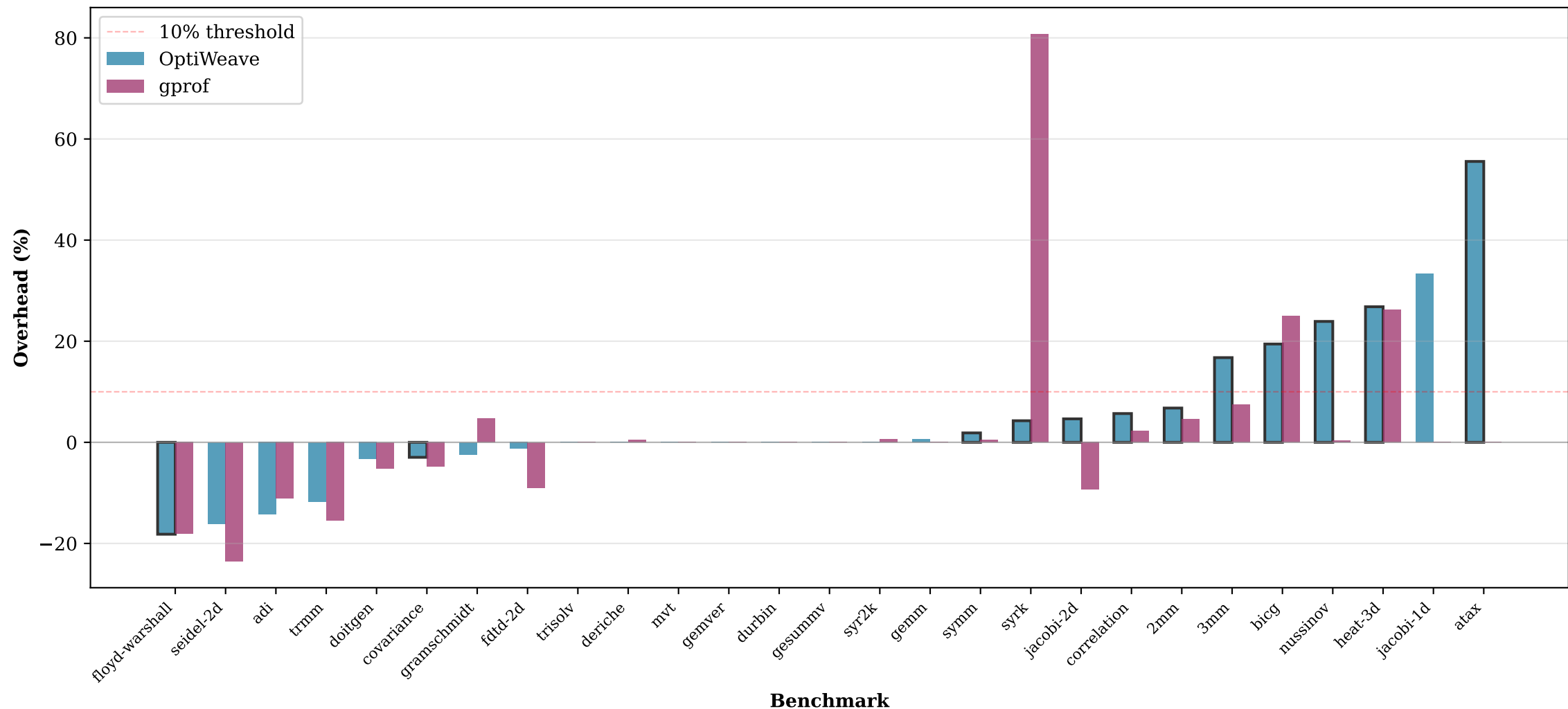
Runtime Overhead Comparison: OptiWeave vs gprof
