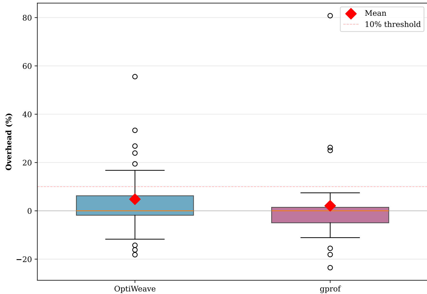
Distribution of Runtime Overhead
