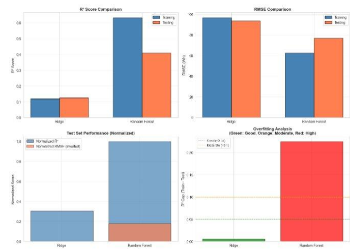
Figure 5: Model Performance Comparison and Overfitting Analysis
