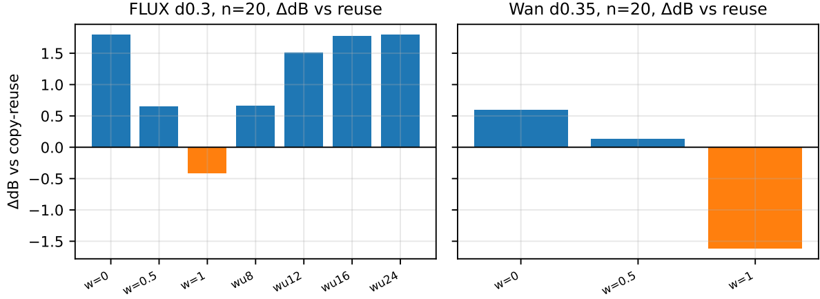
Figure 4: Ablations ( \Delta dB vs copy-reuse). Left: FLUX \delta=0.3 . Right: Wan \delta=0.35 . Pure Chebyshev collapses; pure Taylor wins on short skips; the w=0.5 blend never loses to reuse. Warm-up 12–16 approaches the Taylor limit; window K saturates.
