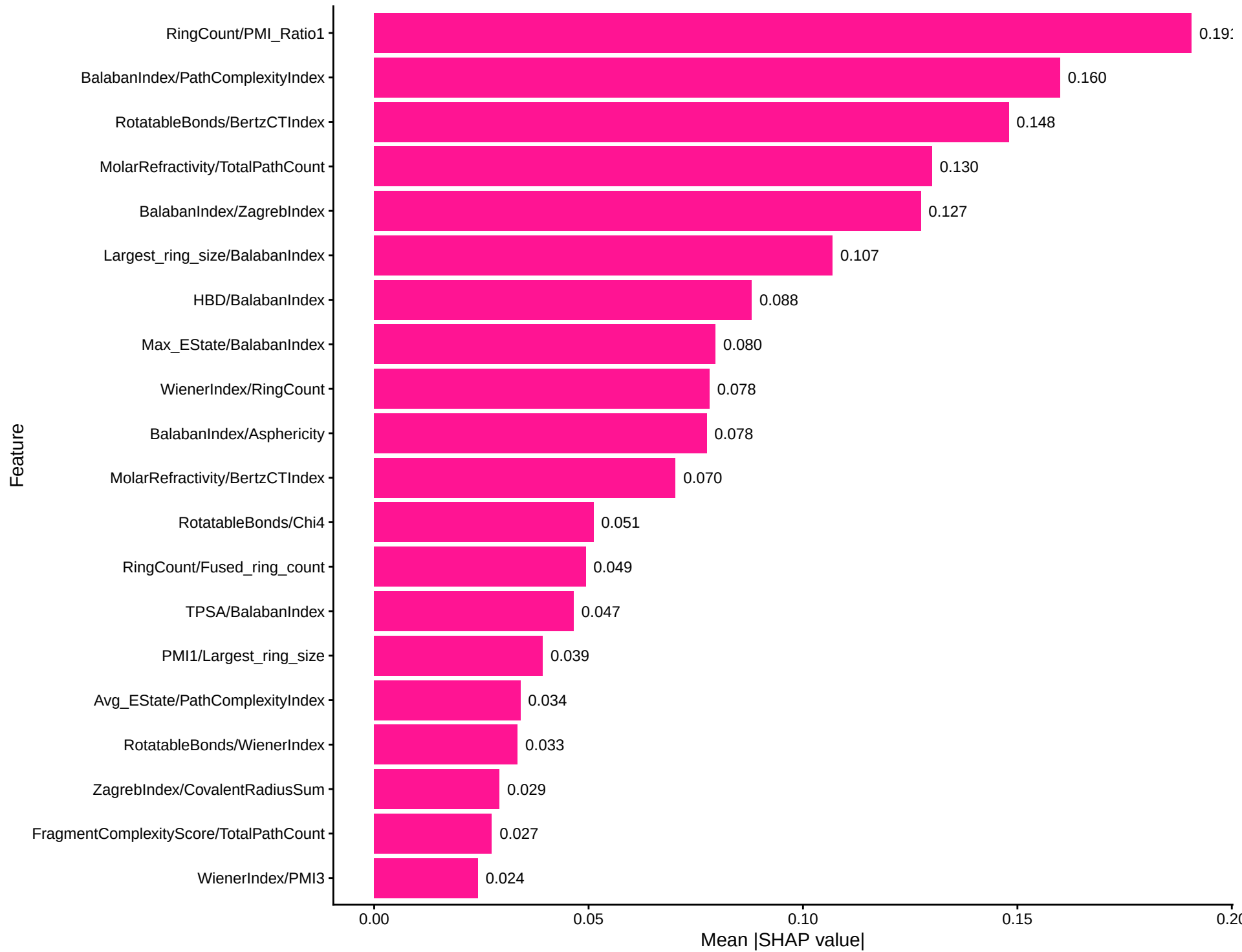
SHAP Importance: AdaBoost Regression
