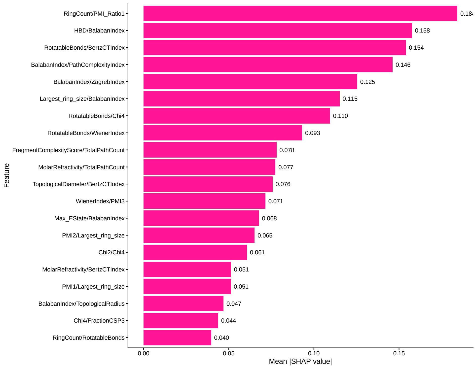
SHAP Top 20 Features: CatBoost Regression
