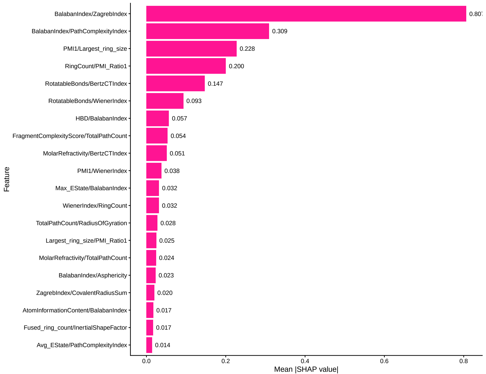
SHAP Top 20 Features: Decision Tree Regression
