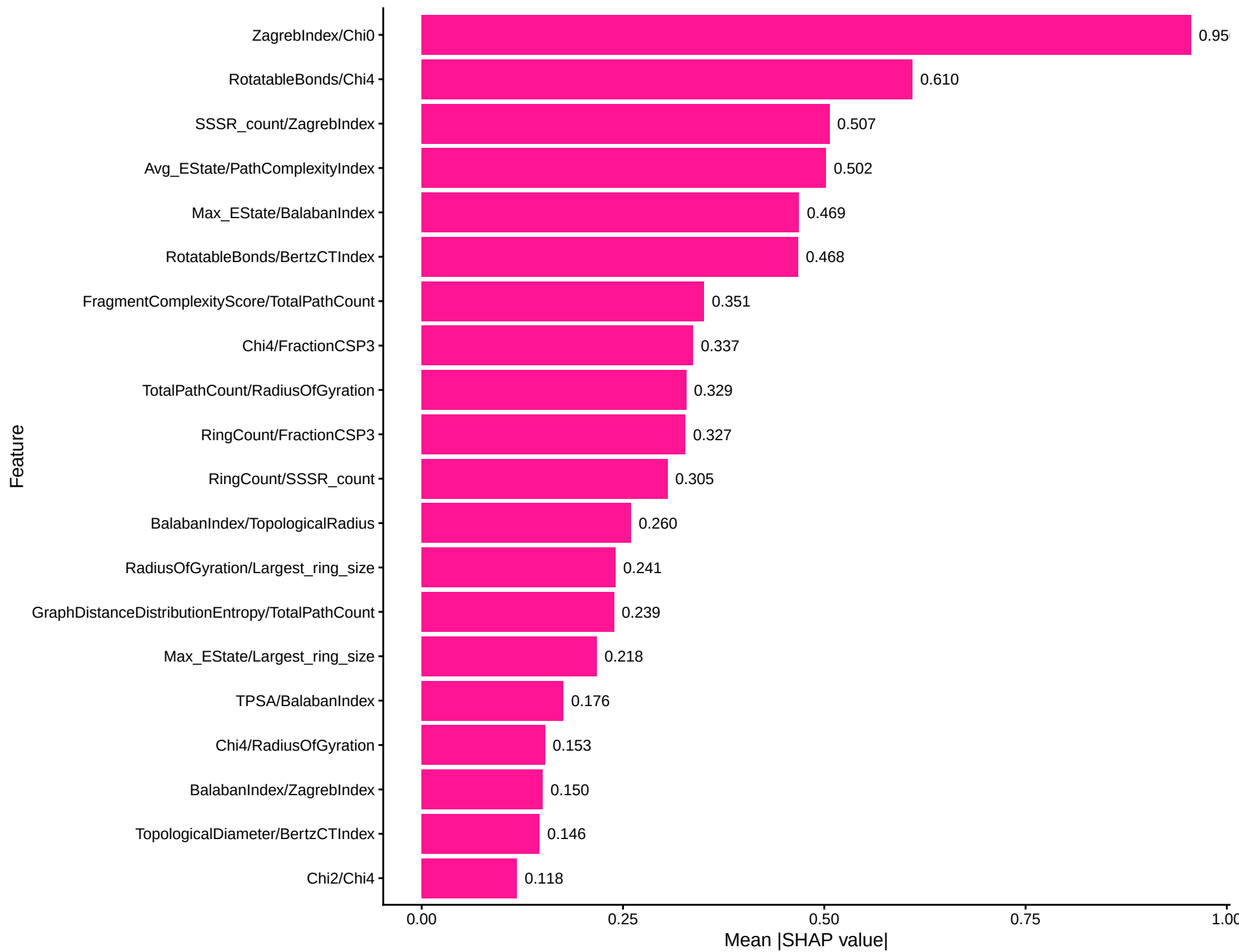
SHAP Top 20 Features: Elastic Net Regression
