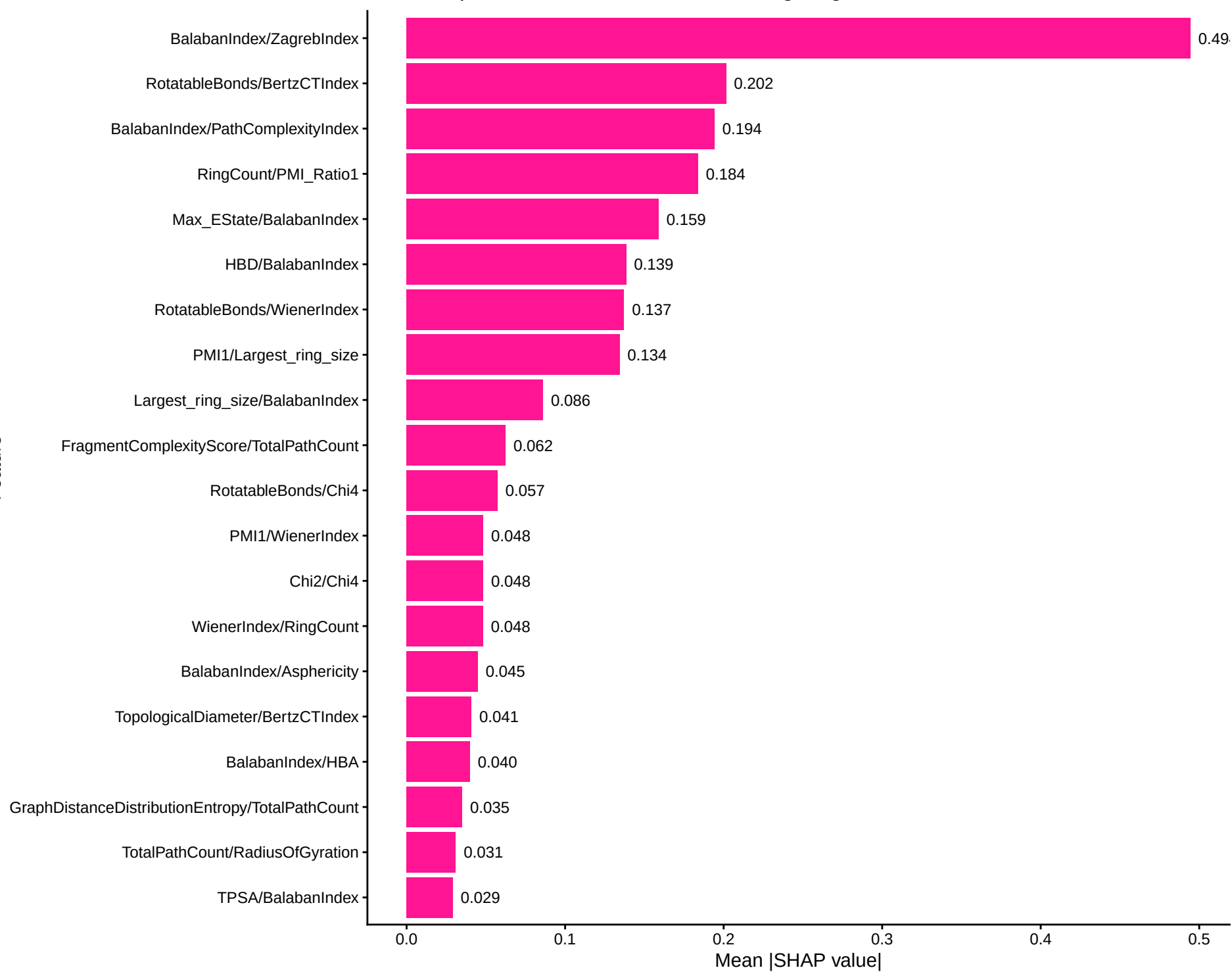
SHAP Top 20 Features: Gradient Boosting Regression
