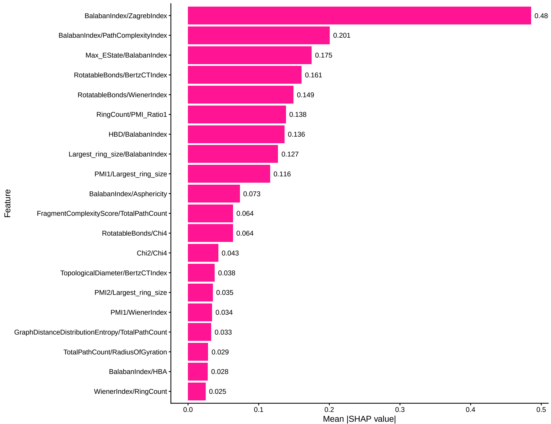
SHAP Top 20 Features: LightGBM Regression
