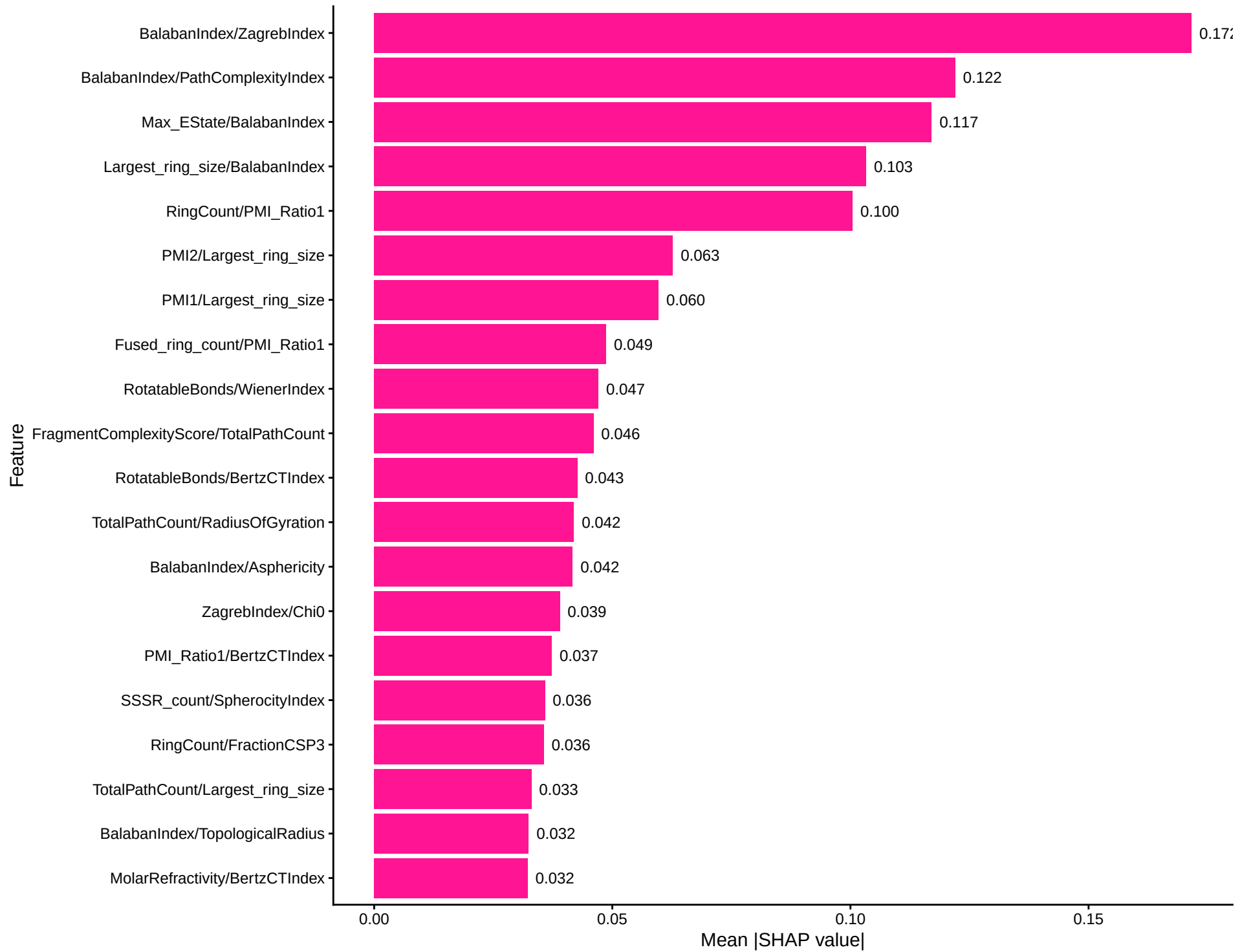
SHAP Top 20 Features: Random Forest Regression
