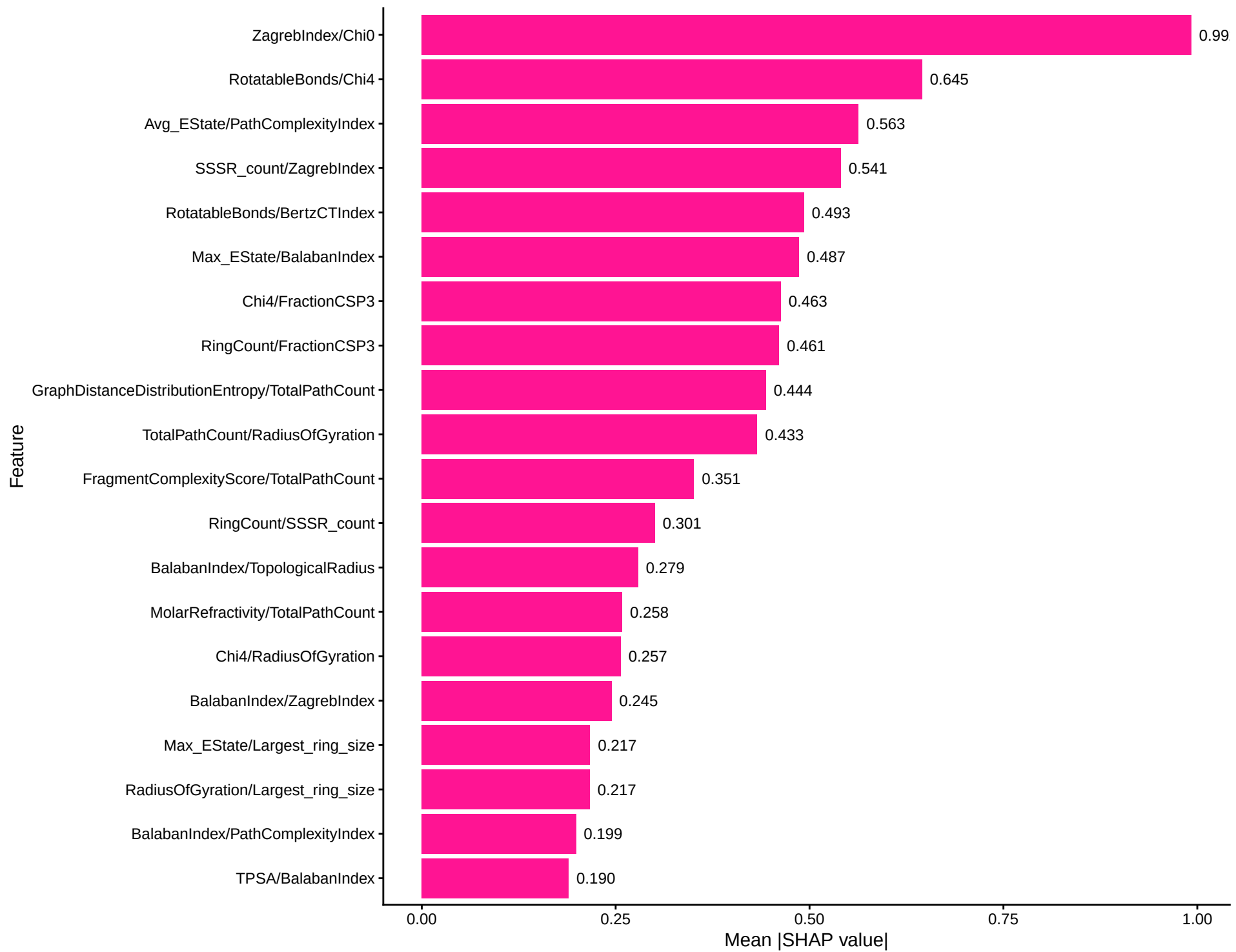
SHAP Top 20 Features: Ridge Regression
