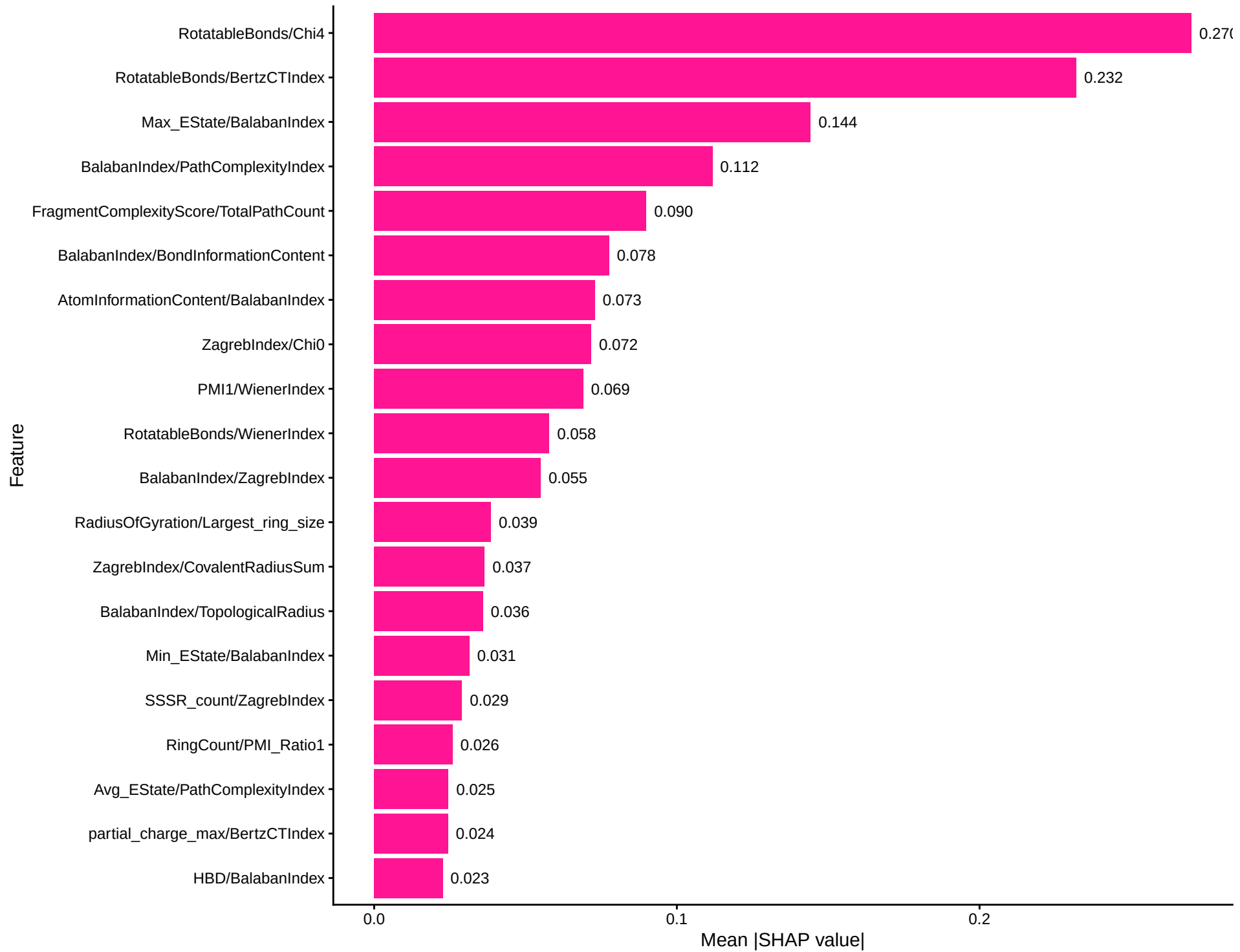
SHAP Top 20 Features: SVR Regression
