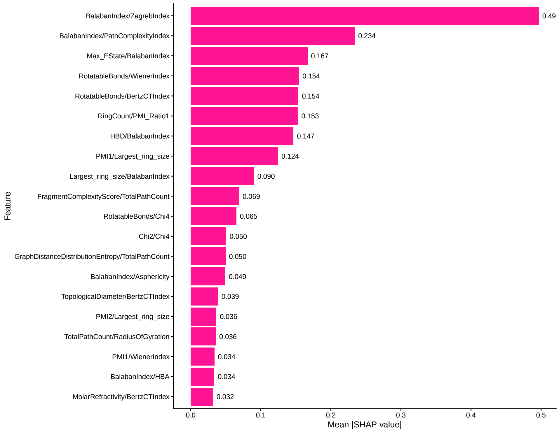
SHAP Top 20 Features: XGBoost Regression
