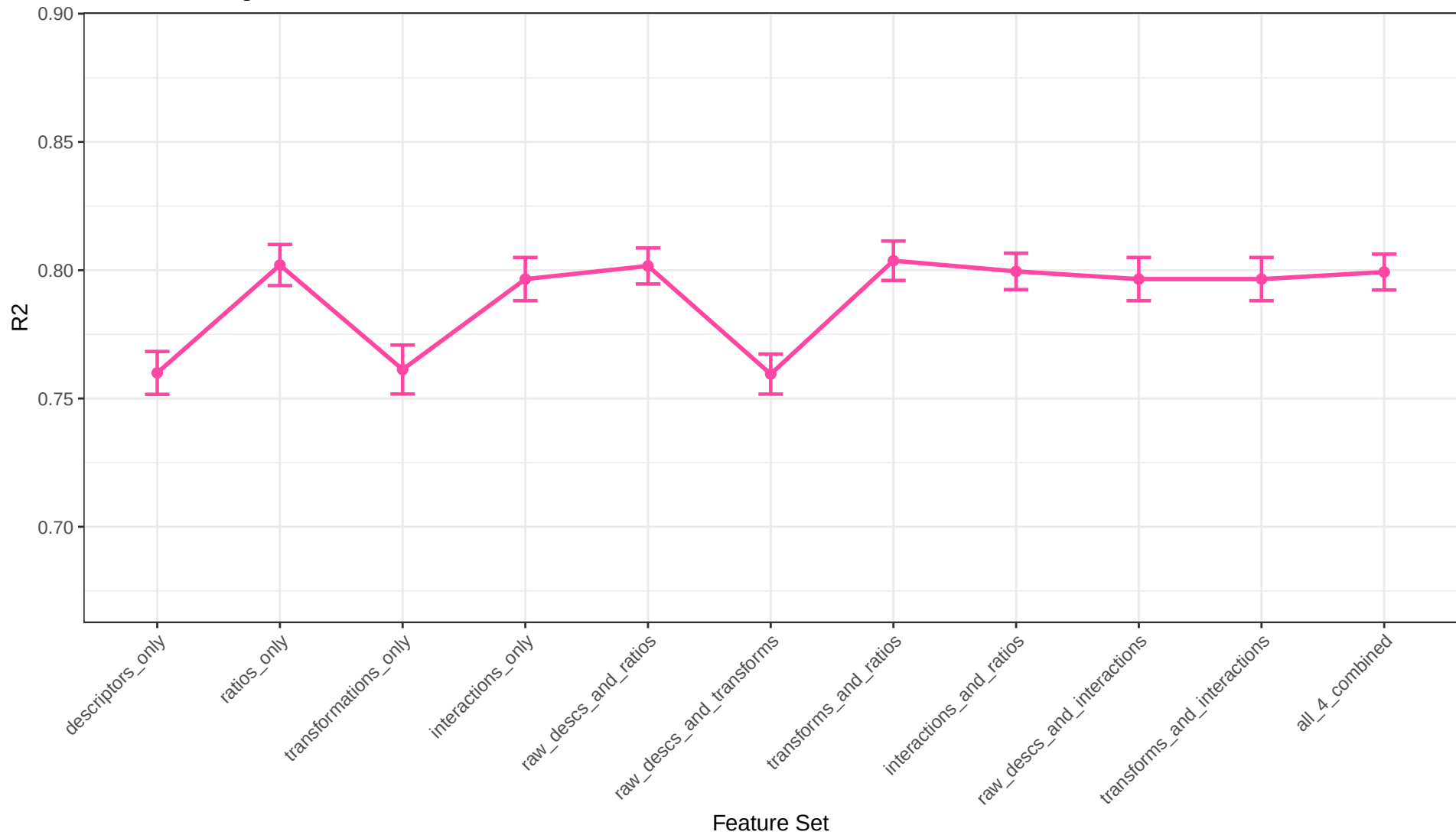
AdaBoost Regression R2 Across Feature Sets
