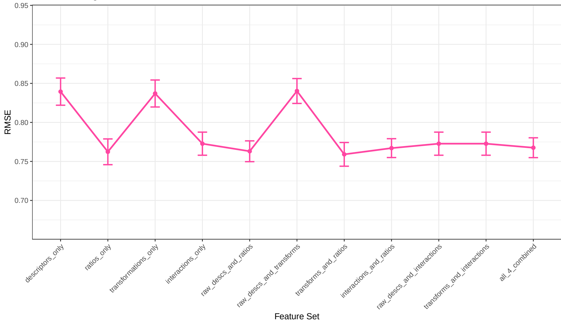
AdaBoost Regression RMSE Across Feature Sets
