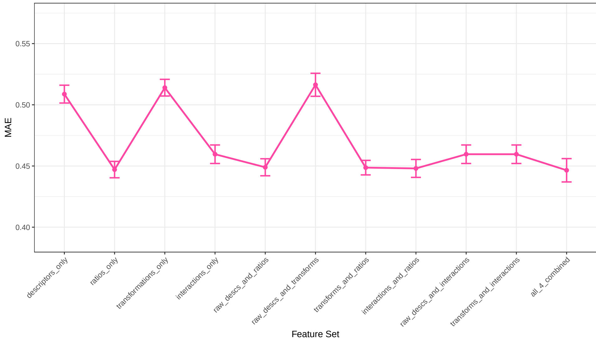
CatBoost Regression MAE Across Feature Sets
