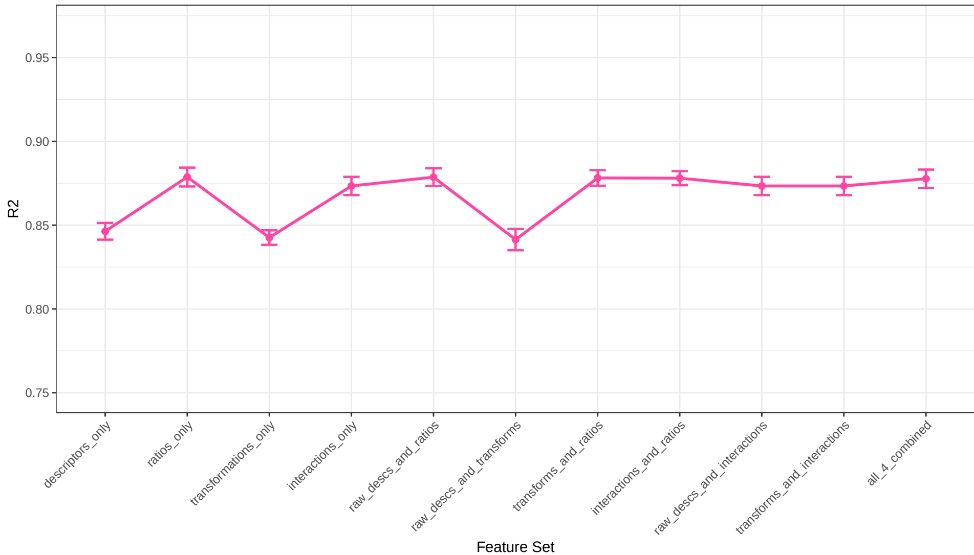
CatBoost Regression R2 Across Feature Sets
