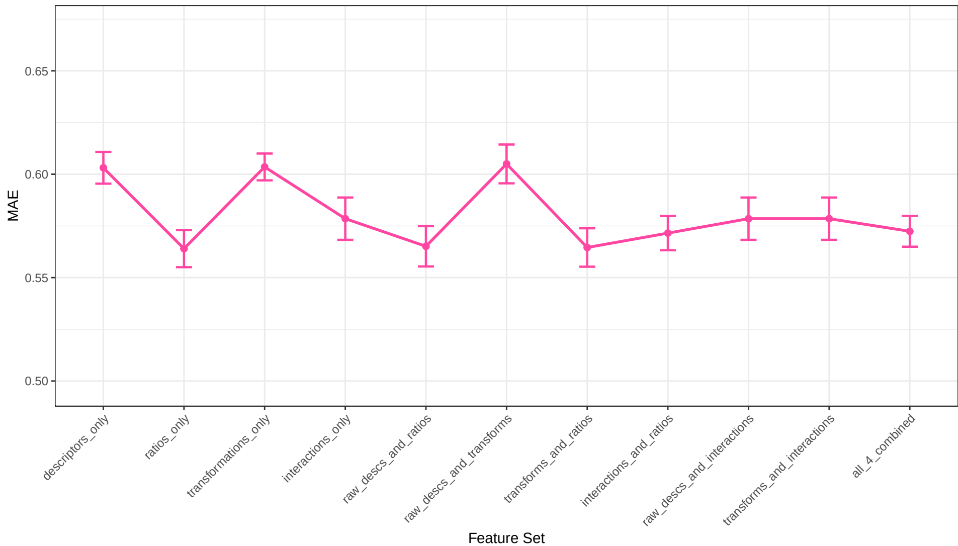
Decision Tree Regression MAE Across Feature Sets
