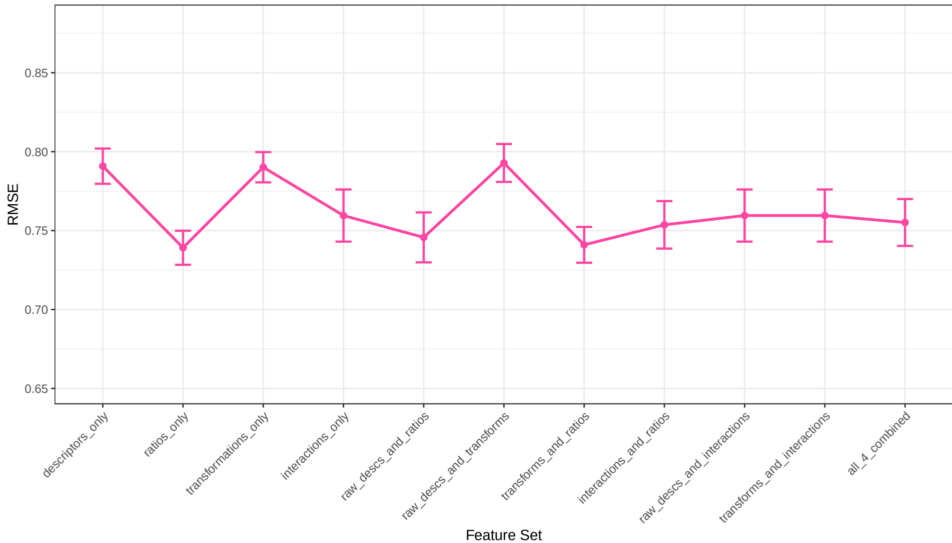
Decision Tree Regression RMSE Across Feature Sets
