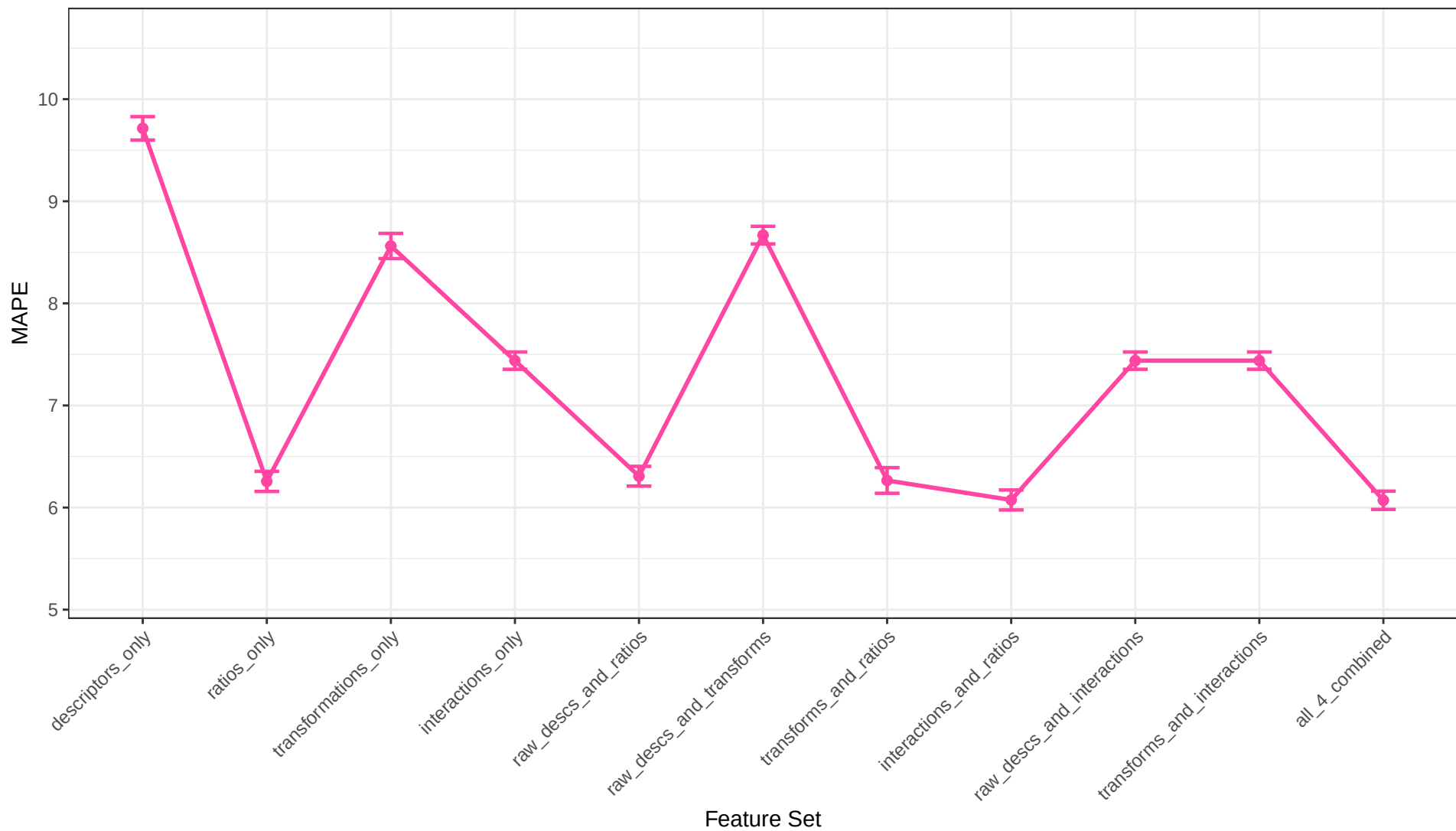
Elastic Net Regression MAPE Across Feature Sets
