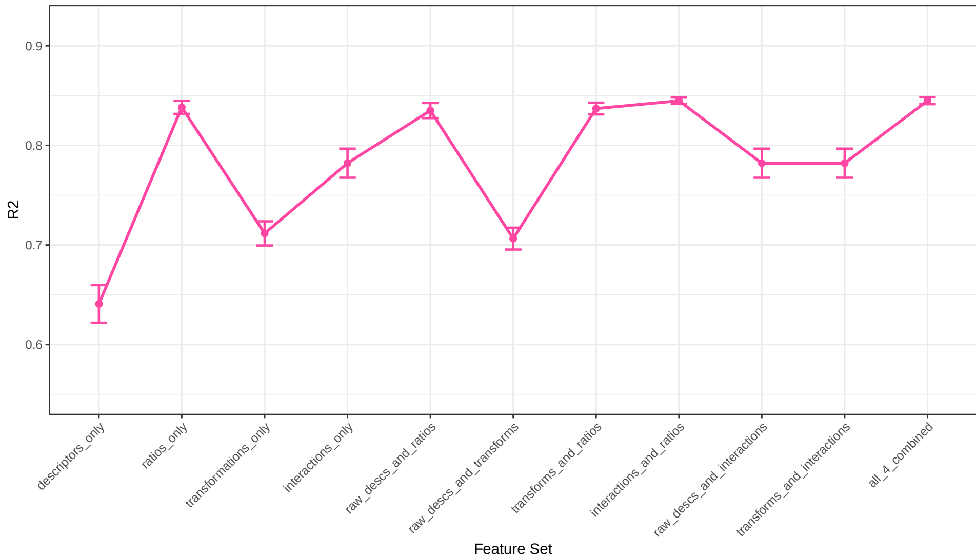
Elastic Net Regression R2 Across Feature Sets
