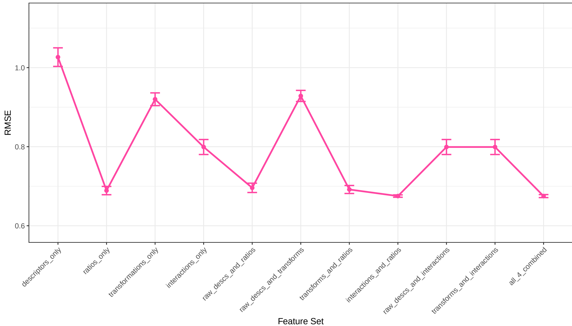
Elastic Net Regression RMSE Across Feature Sets
