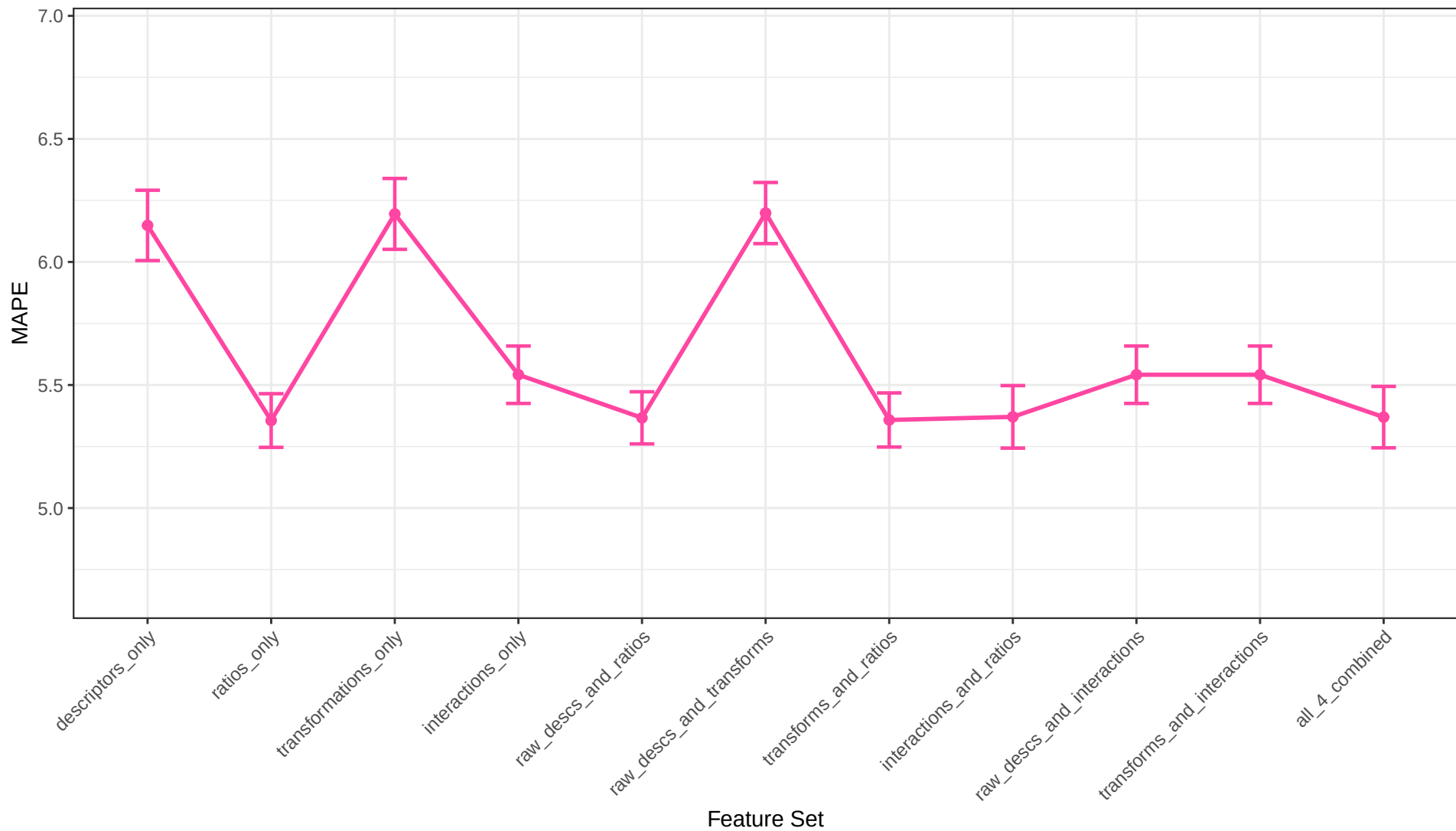
Gradient Boosting Regression MAPE Across Feature Sets
