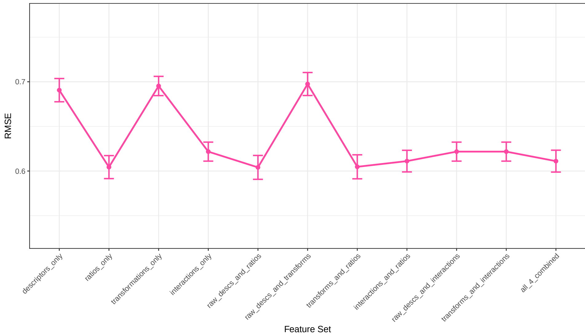
Gradient Boosting Regression RMSE Across Feature Sets
