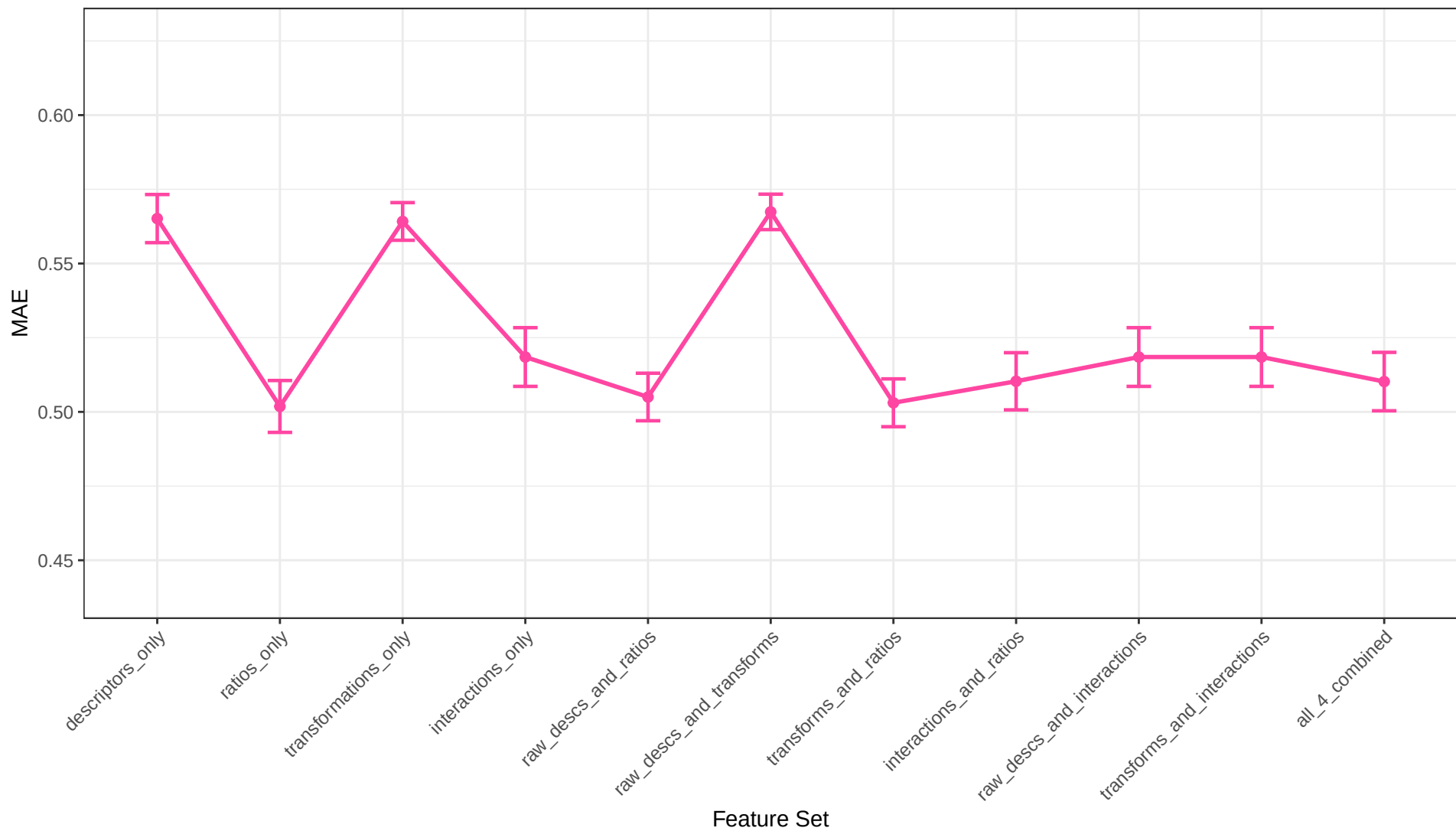
K-Nearest Neighbours Regression MAE Across Feature Sets
