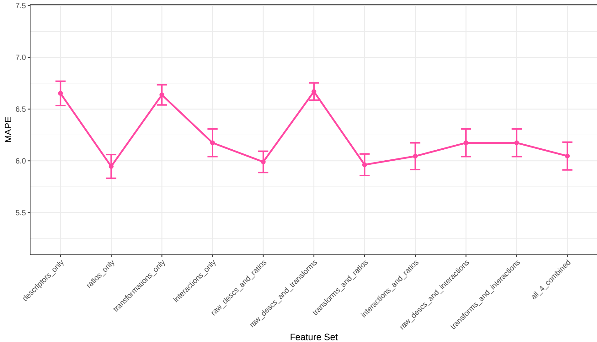
K-Nearest Neighbours Regression MAPE Across Feature Sets
