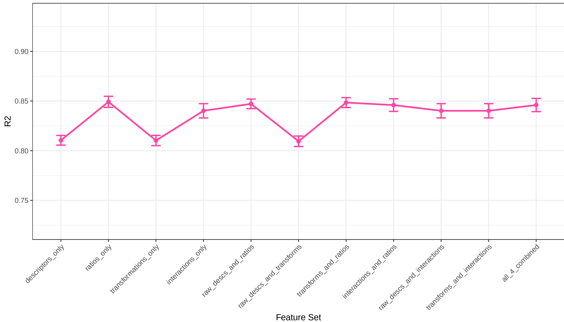
K-Nearest Neighbours Regression R2 Across Feature Sets
