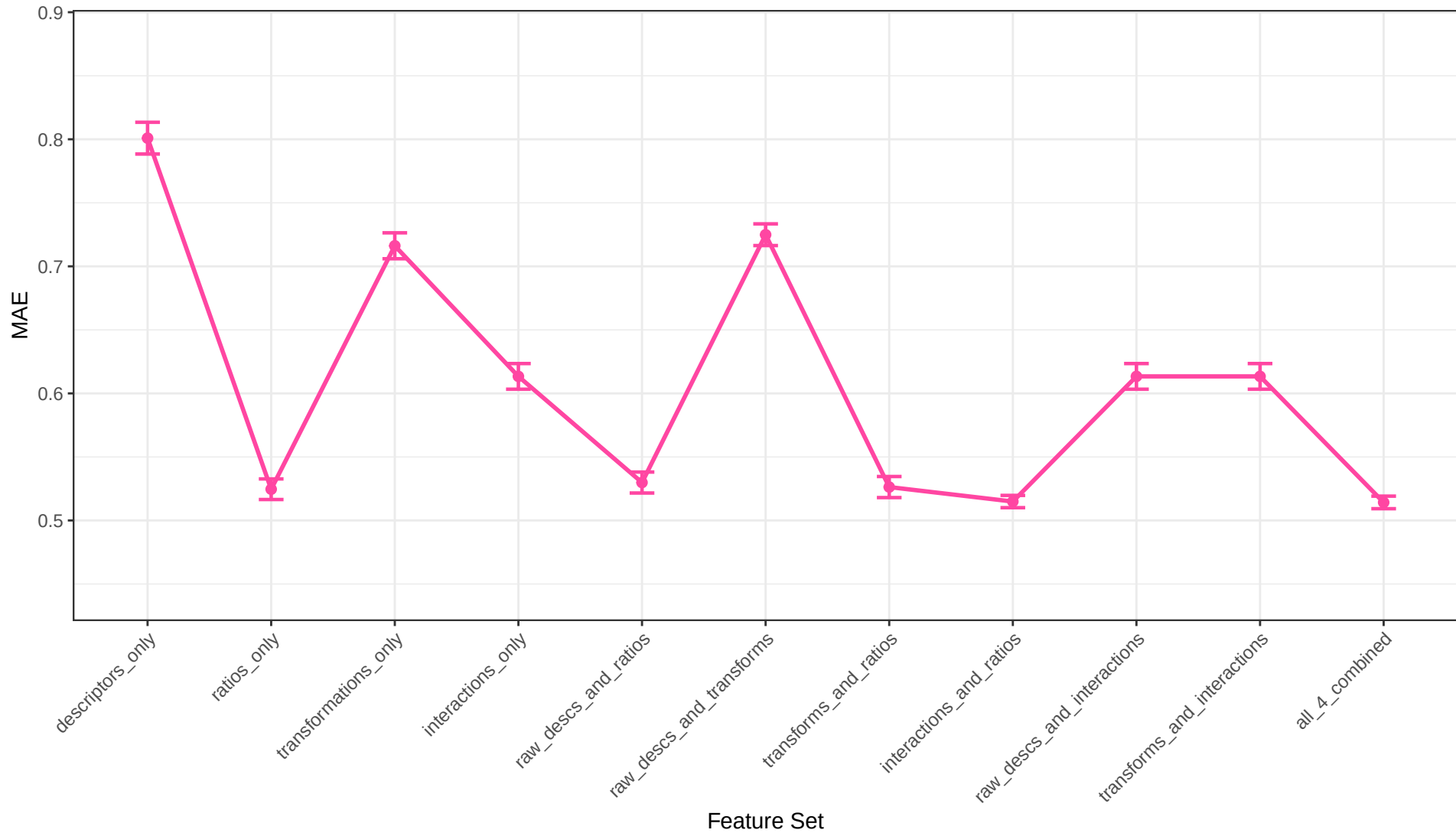
Lasso Regression MAE Across Feature Sets
