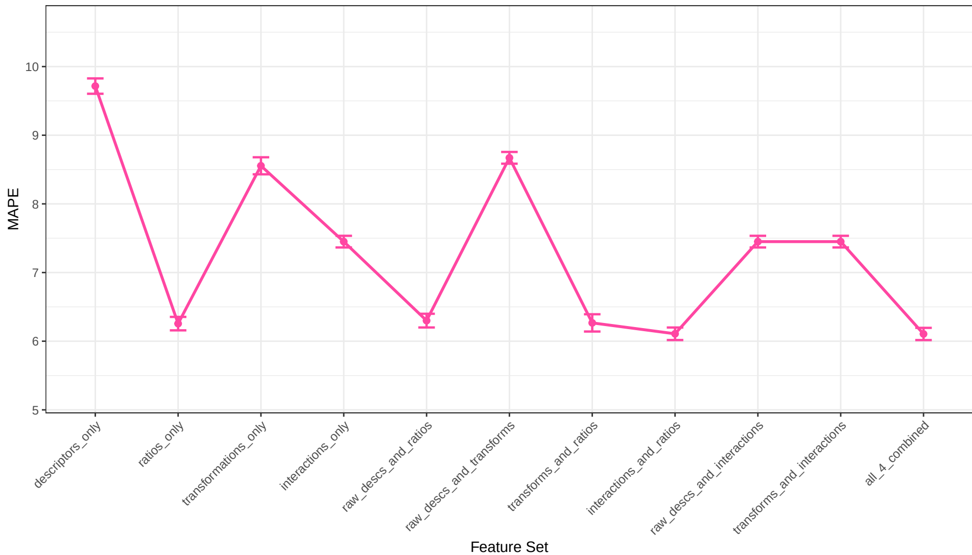
Lasso Regression MAPE Across Feature Sets
