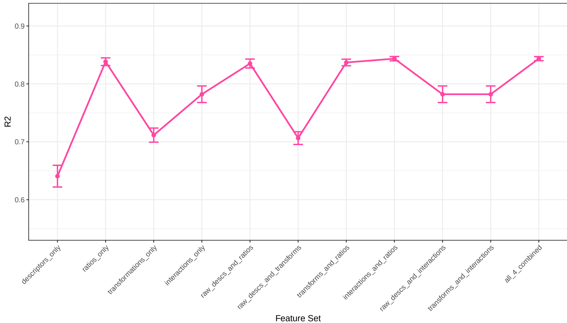
Lasso Regression R2 Across Feature Sets
