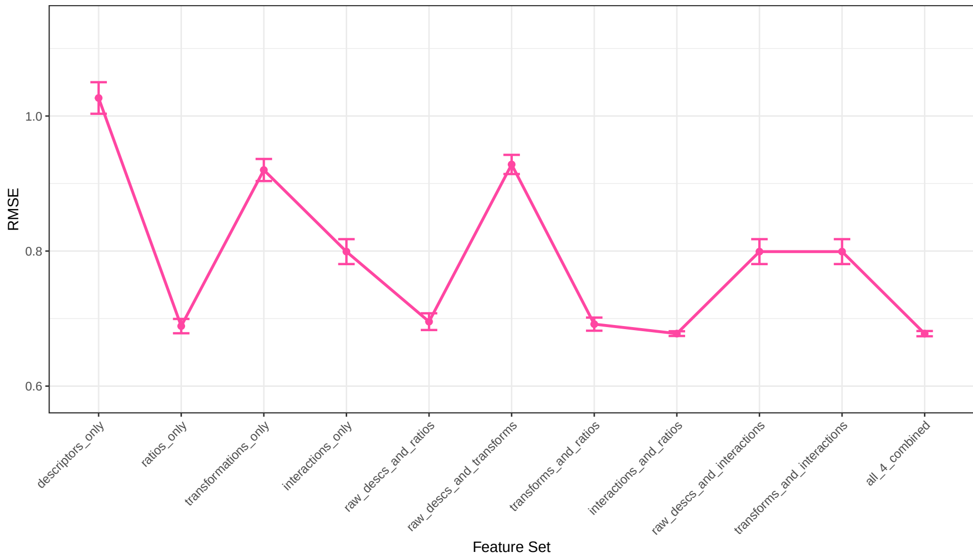
Lasso Regression RMSE Across Feature Sets
