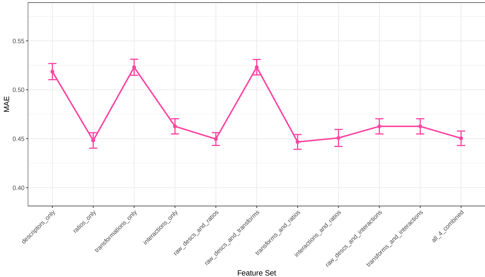
LightGBM Regression MAE Across Feature Sets
