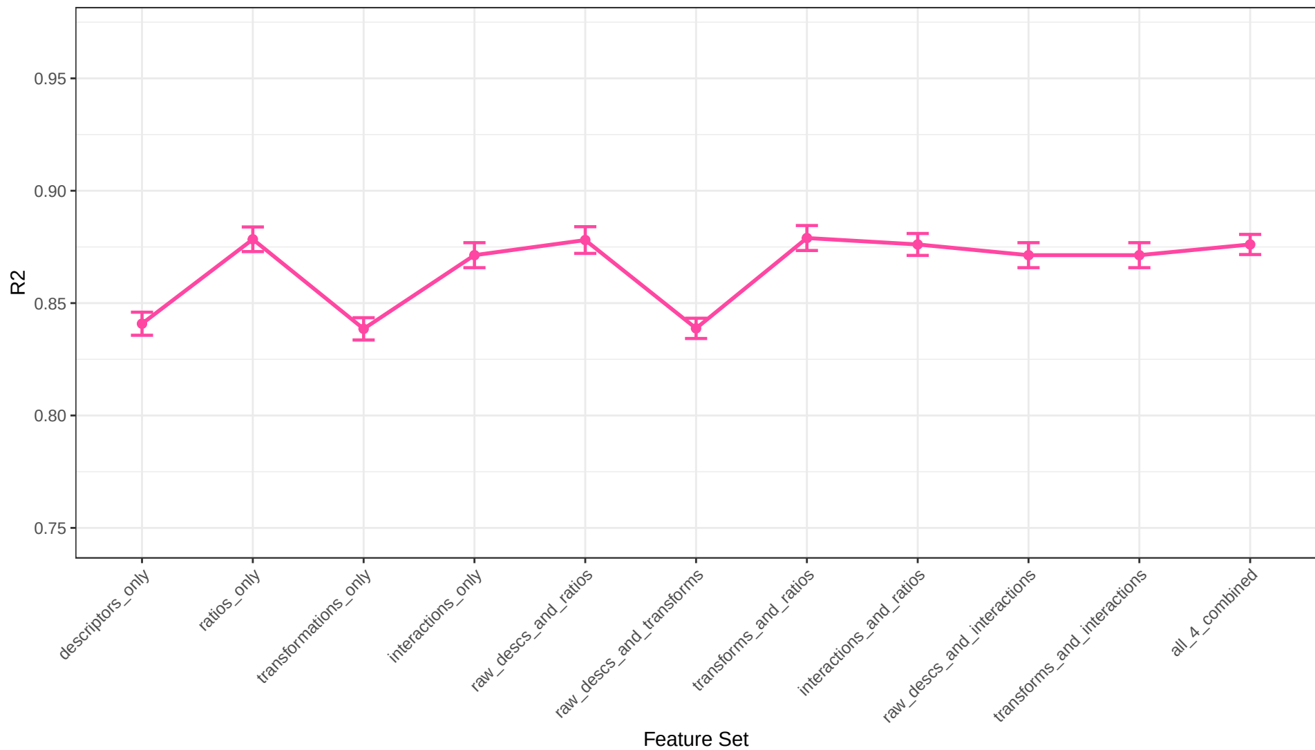
LightGBM Regression R2 Across Feature Sets
