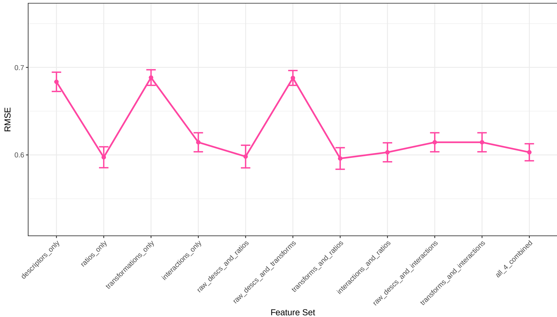
LightGBM Regression RMSE Across Feature Sets
