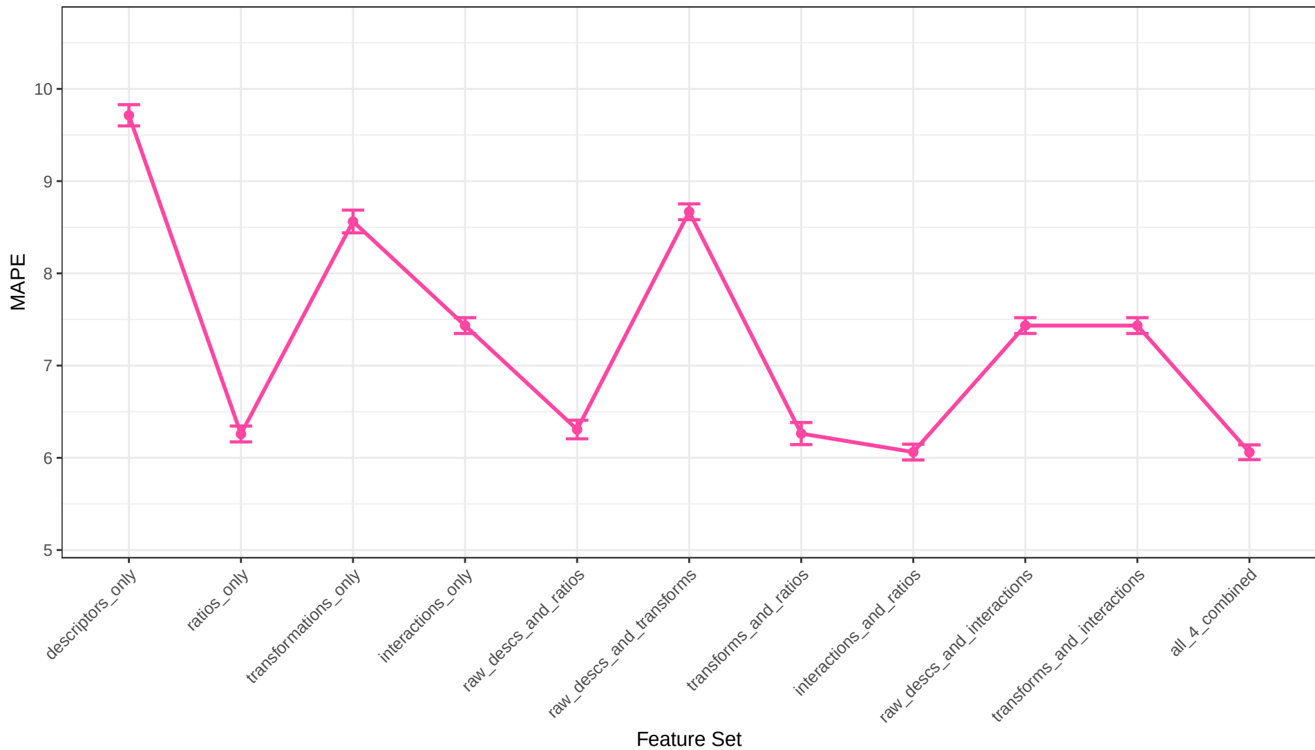
Linear Regression MAPE Across Feature Sets
