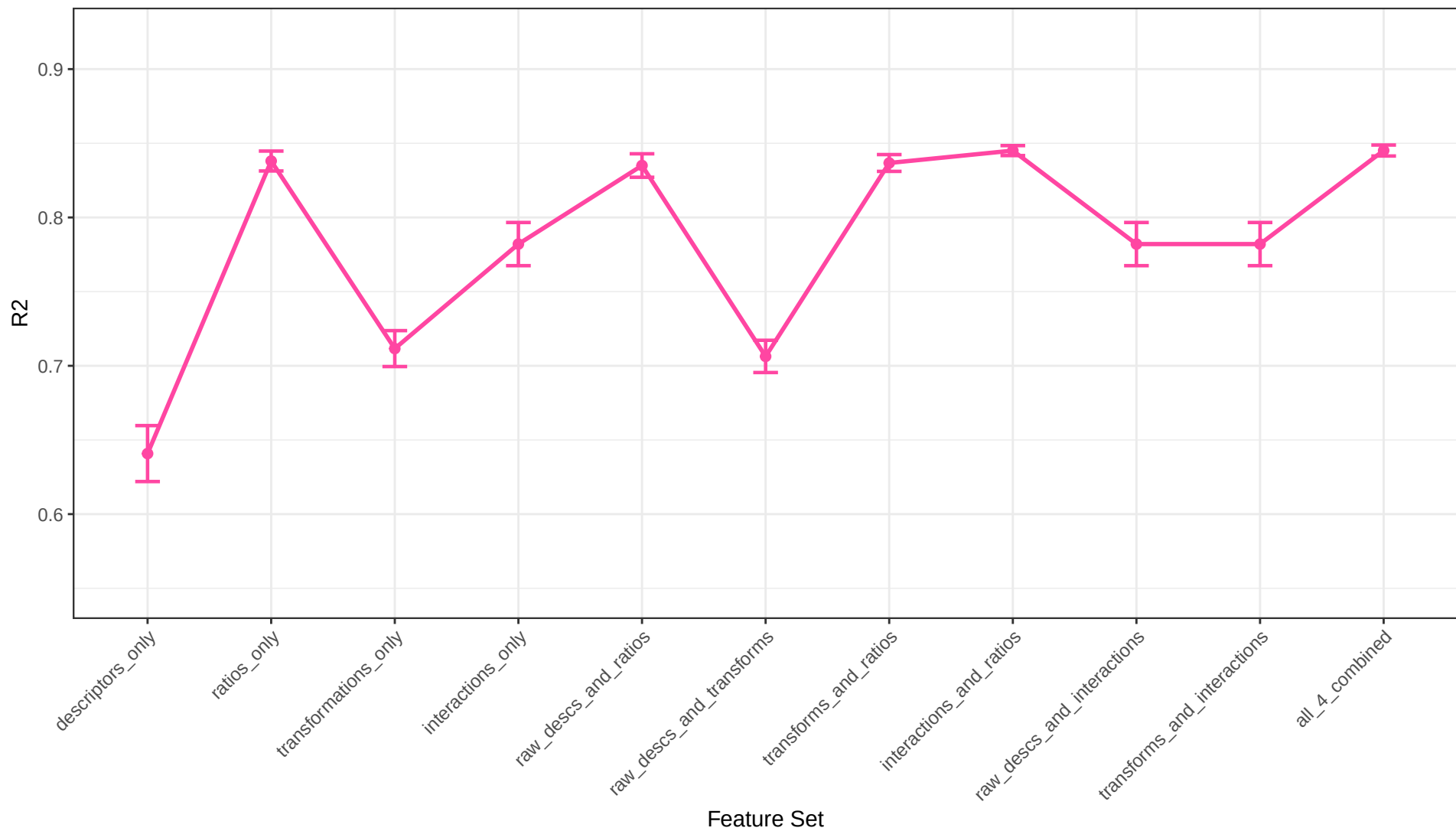
Linear Regression R2 Across Feature Sets
