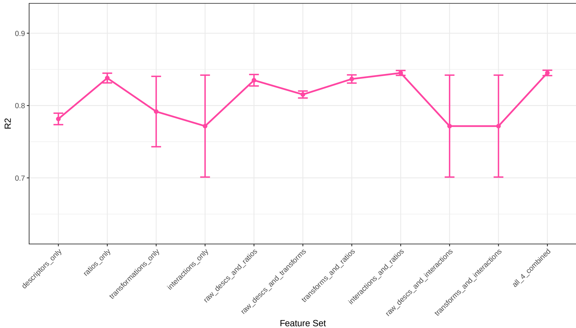
Polynomial Regression R2 Across Feature Sets
