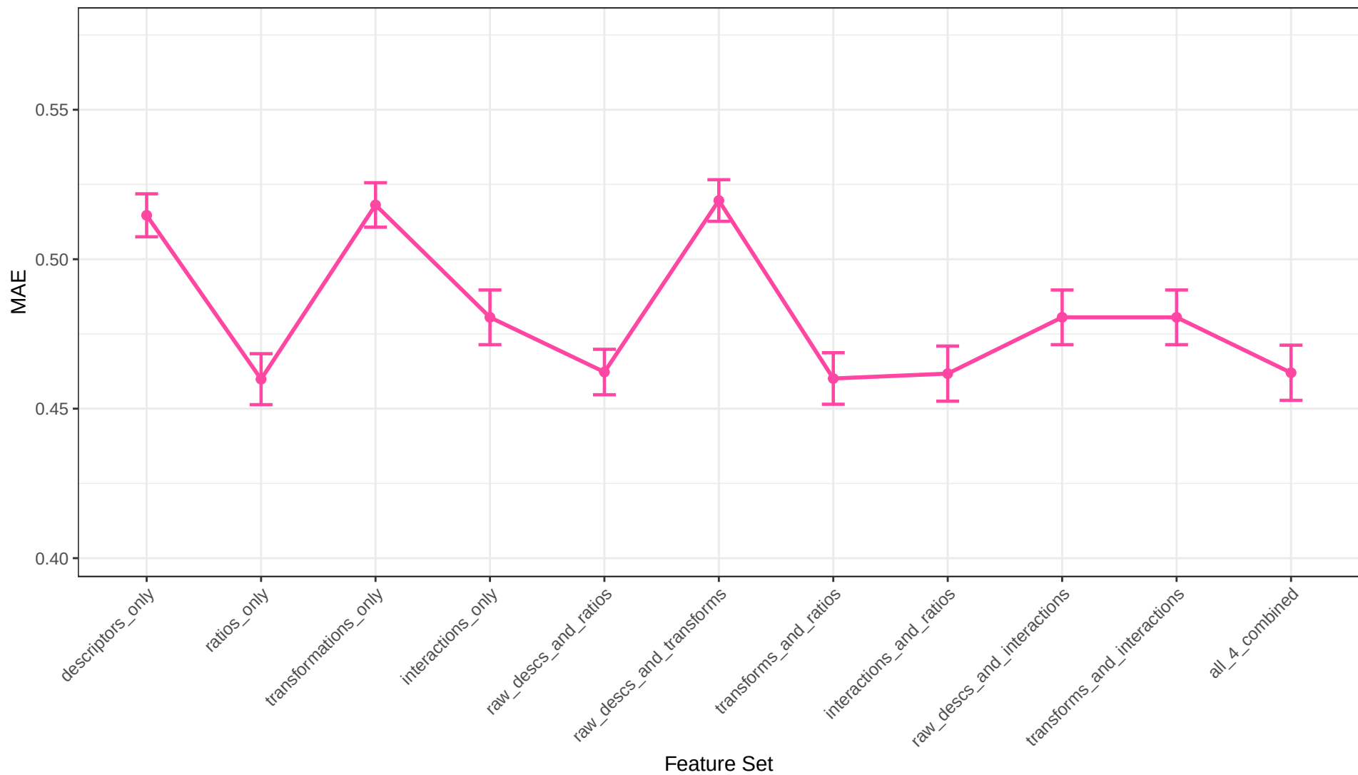
Random Forest Regression MAE Across Feature Sets
