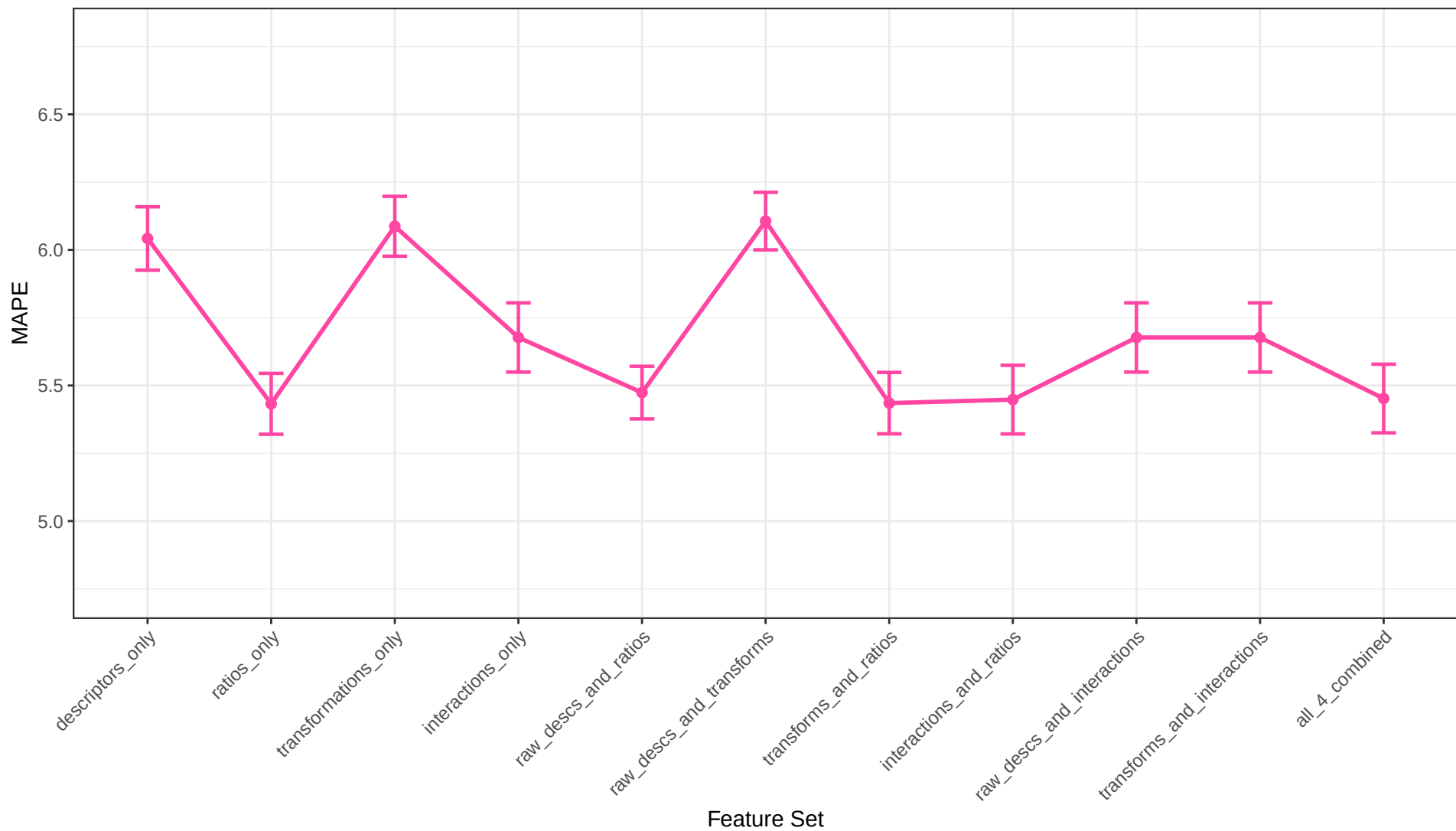
Random Forest Regression MAPE Across Feature Sets
