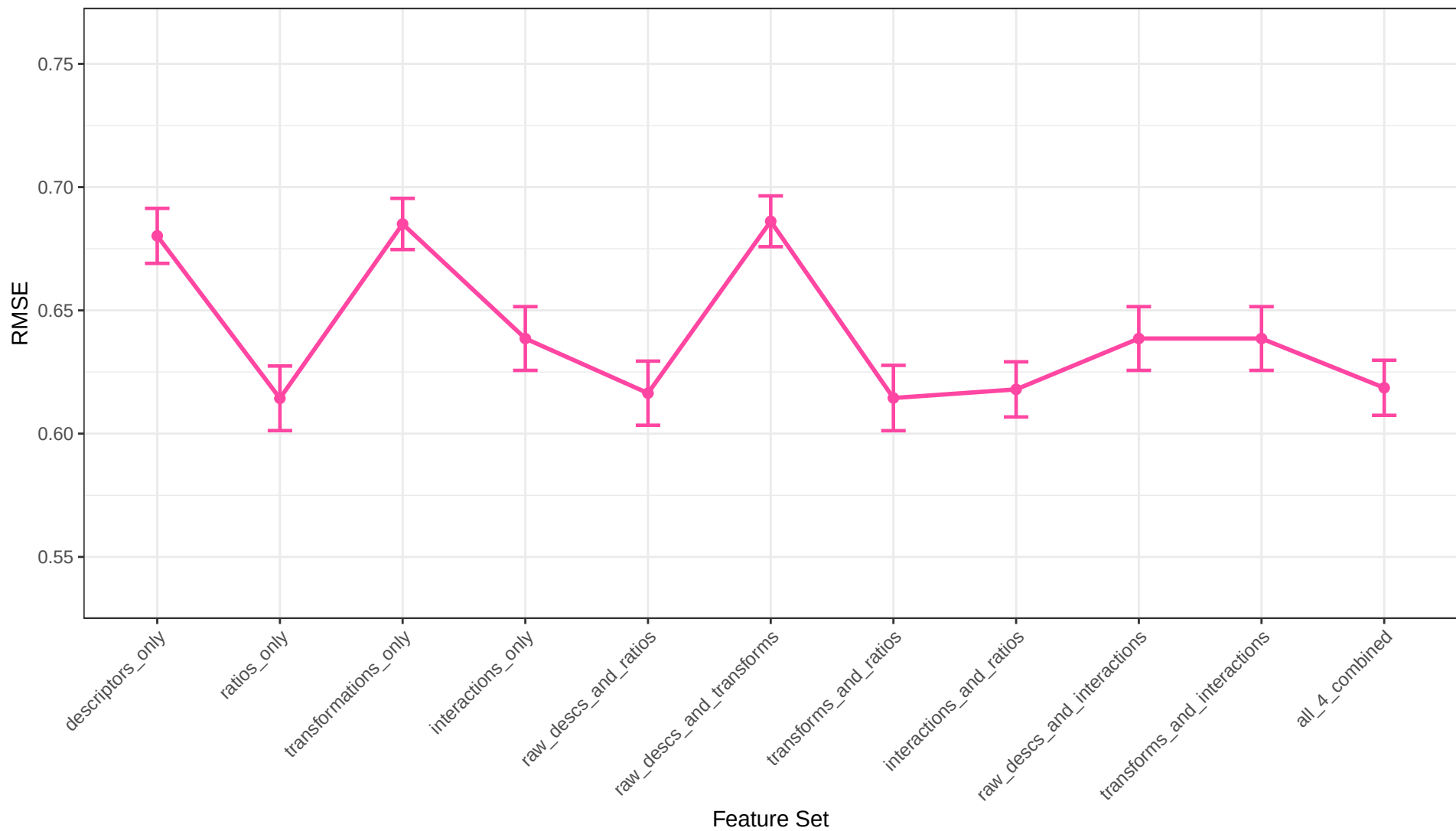
Random Forest Regression RMSE Across Feature Sets
